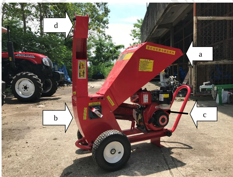
Figure 1. Parts of the JHT SCH-1 Biomass Shredder (a) Hopper, (b) Shredding Chamber, (c) Prime mover, and (d) Output chute
